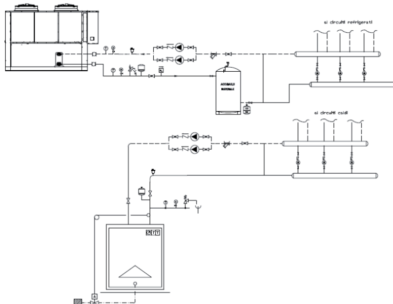
PRINCIPLE DIAGRAM Heating-cooling unit with con- densing boiler and chiller.
