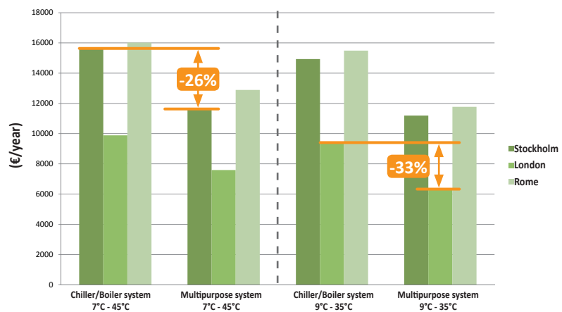
ESTIMATION OF OPERATING COSTS (€/YEAR)
