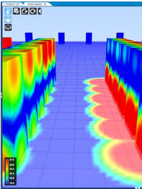
The Trellis™ Thermal System Manager
